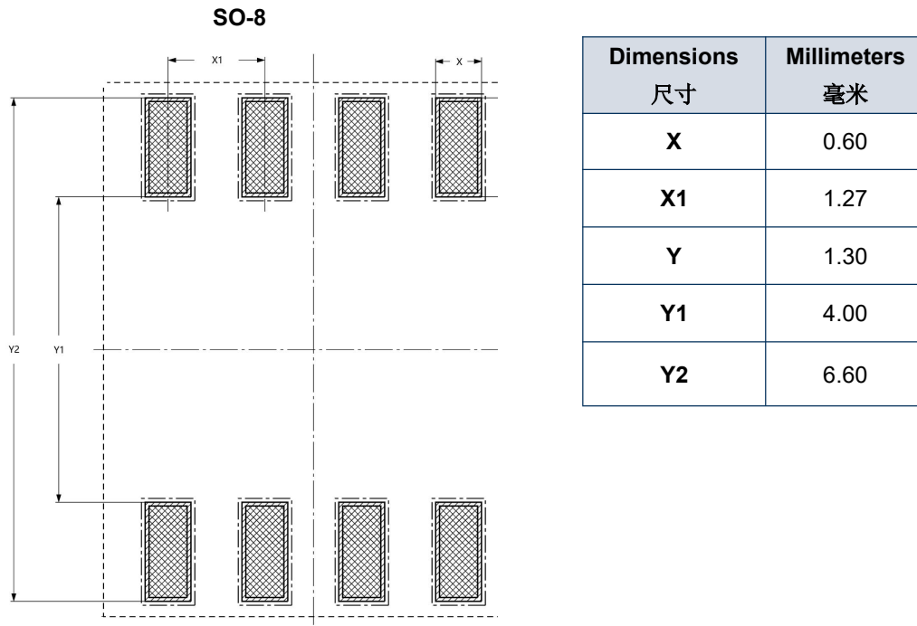
Fig. Soldering footprint for SO-8
