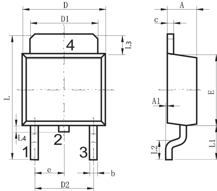
TO-252
