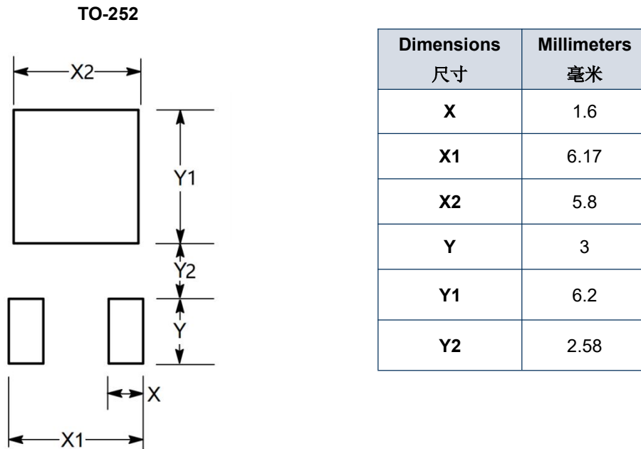
Fig. Soldering footprint for TO-252
